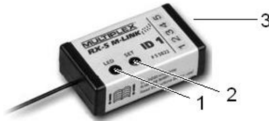
Fig. 3: receptor RX-5 light M-LINK ID 1
