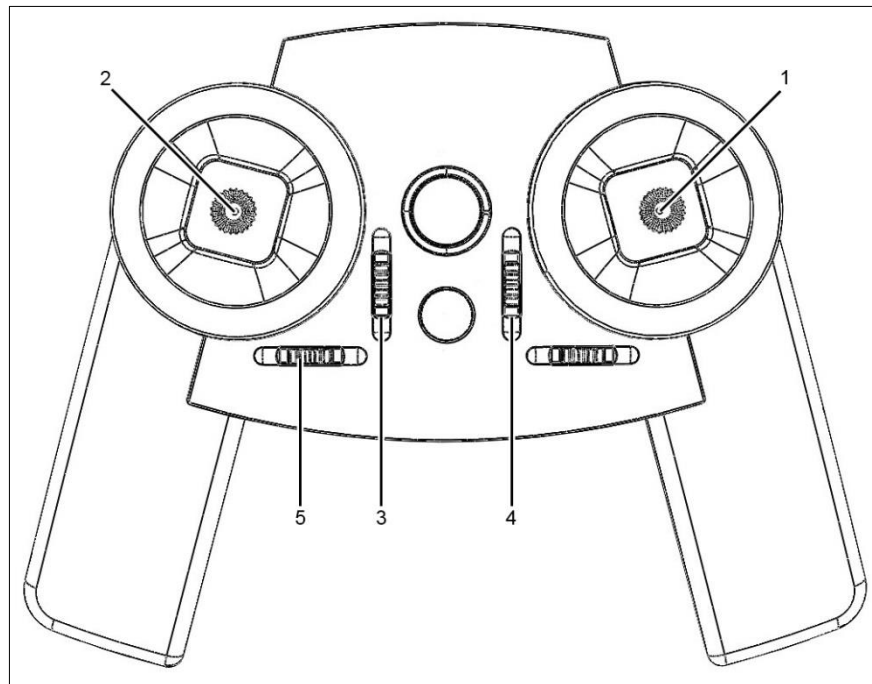
Fig. 6: SMART SX FLEXX transmitter – actuator and servo assignment
